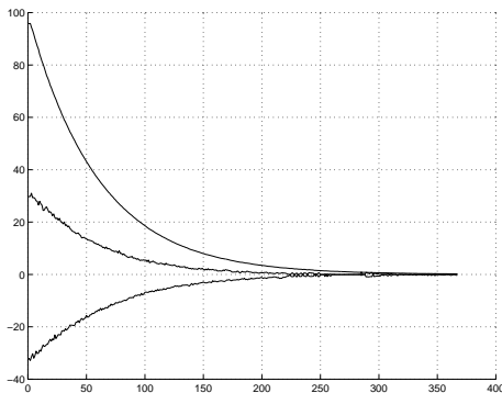
Fig. 11. Rotation u\theta (dg) versus iteration number
