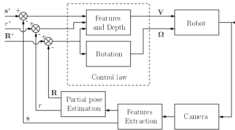
Fig. 6. Block diagram of the 2D 1/2 visual servoing
